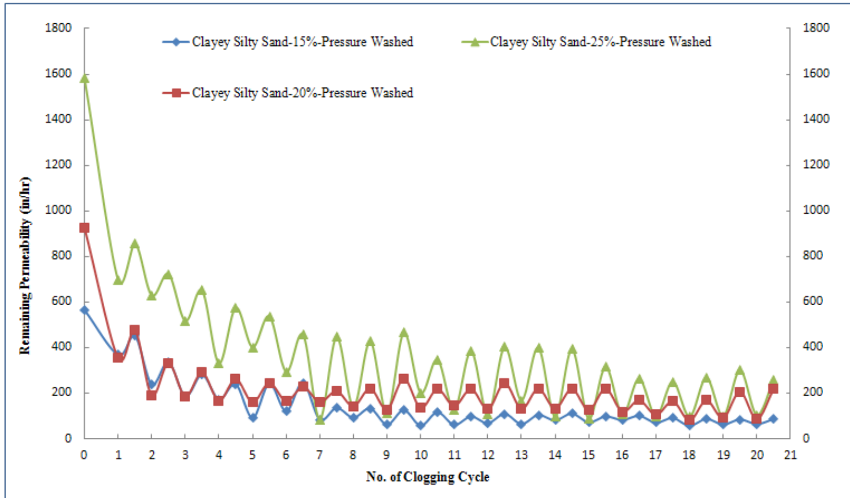
Figure 4-13. Permeability Coefficient of Permeability of Specimens Subjected to Clayey Silty Sand Sediments and Cleaned by Pressure Washing
