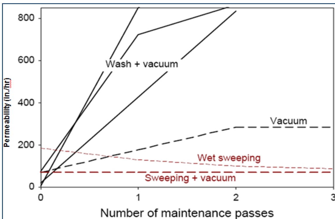
Figure 2-30. The Permeability Recovery by Different Rehabilitation Methods (Adopted from [38])
